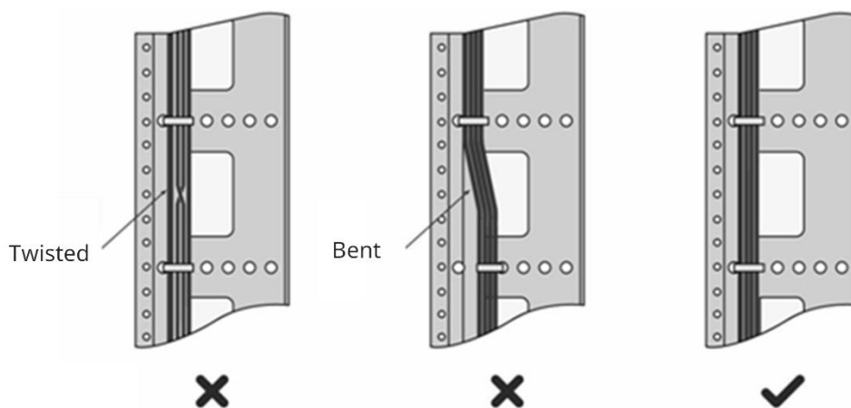
Figure 6-1 Binding Cables (1)
