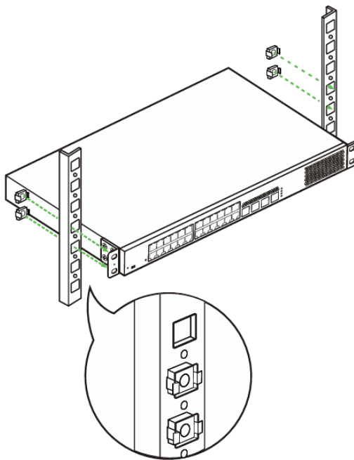
Figure 3-1 Securing Rack-Mount Brackets to the Rack (1)
