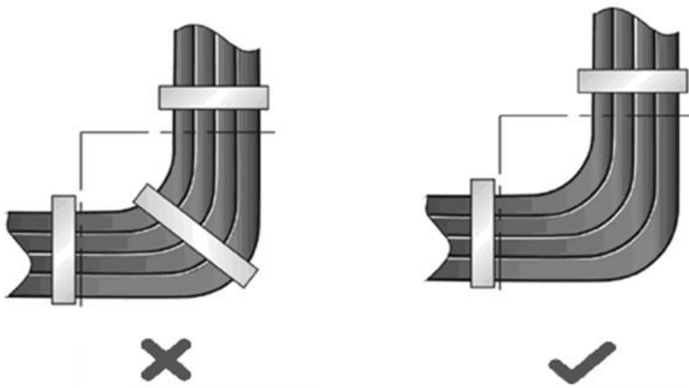
Figure 6-3 Binding Cables (3)
