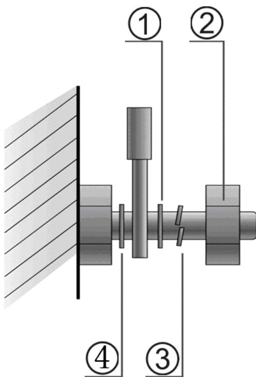
Figure 6-4 Cable Fastening
